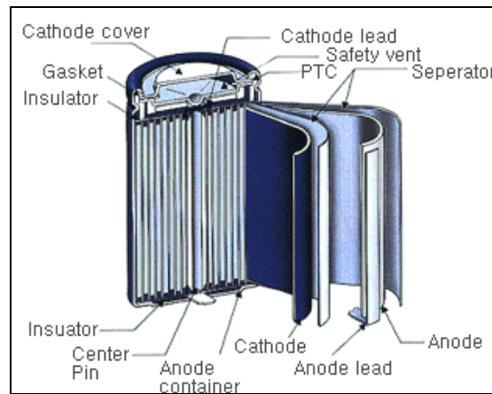
Figure 3. Cross-Section of a Cylindrical Li-ion Cell
